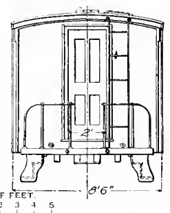
Fig. 86. End Elevation.
